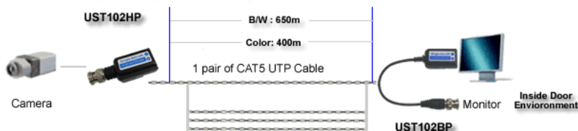
1000ft Passive Video BALUN Transceiver CCTV System Installation Configuration Diagram
